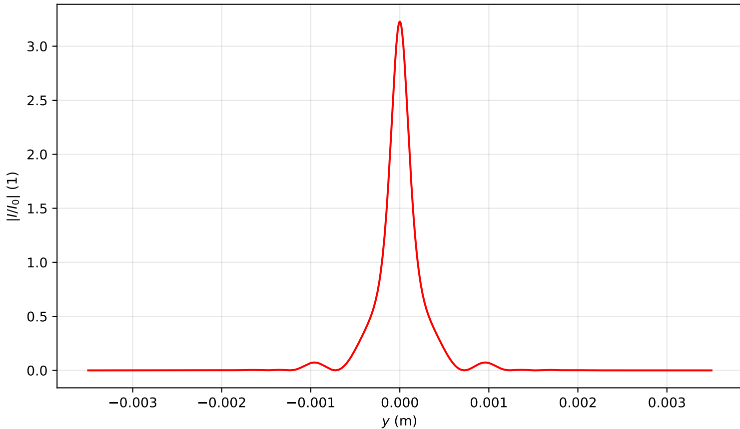
Intensity profile I(x = 0, y, z = 1.433)/I_0 , \text{Pin}=3.0\text{Pcr} , artificial time
